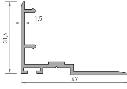
2022 KENET PROFİLİ 0,390 kg/mt
