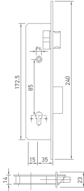
Geniş Kilit (Dilli) Wide Type Lock (Bolt)
