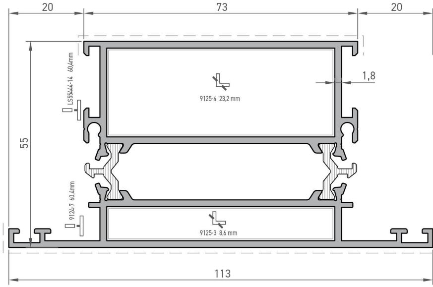
Baza Profili Base Profile
