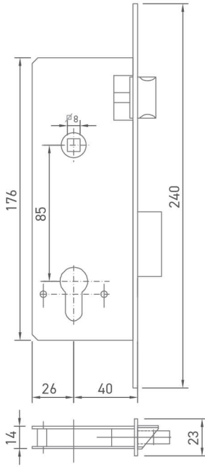
Geniş Kilit (Dilli) Wide Type Lock (Bolt)
