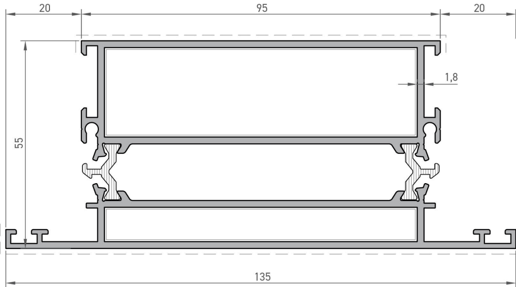
Baza Profili Base Profile
