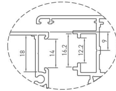
PVC Kanallı Kesit 9 mm PVC Groove Section 9 mm
