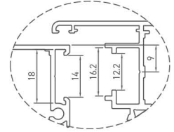
PVC Kanallı Kesit 9 mm PVC Groove Section 9 mm
