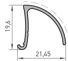
Damlalık Profili Drip Profile
