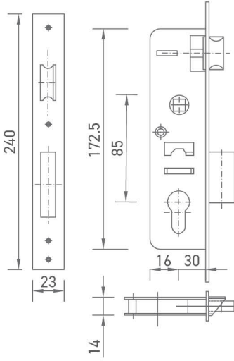
KT02-3 DİLLİ KİLİT
