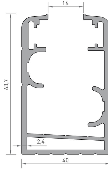
4222 KASA PROFİLİ 1,540 kg/mt
