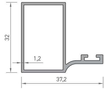
V.CB. 109 YAN KASA PROFİLİ 0,426 kg/mt
