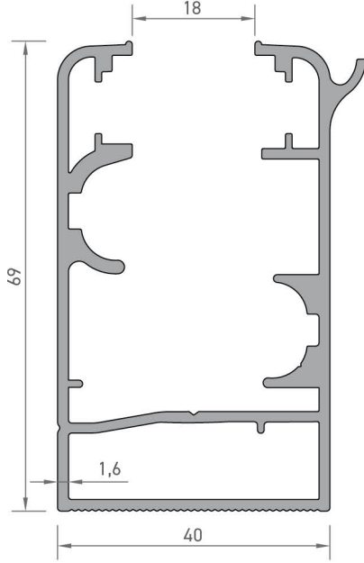
V.CB. 101 KASA PROFİLİ 1,370 kg/mt
