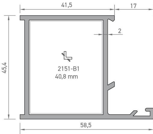
2185 GENİŞ KASA PROFİLİ 1,025 kg/mt
