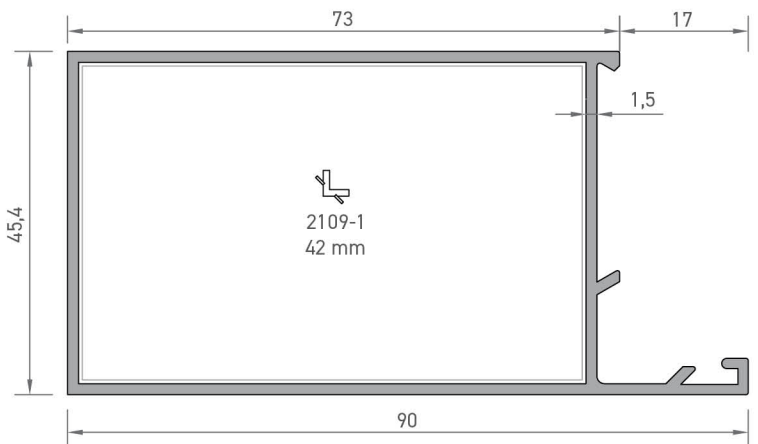
2197 BAZA KASA PROFİLİ 1,025 kg/mt
