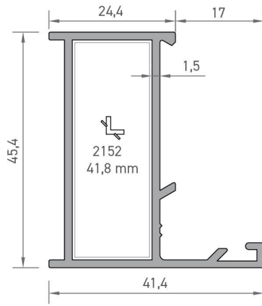
2203 DAR KASA PROFİLİ 0,660 kg/mt
