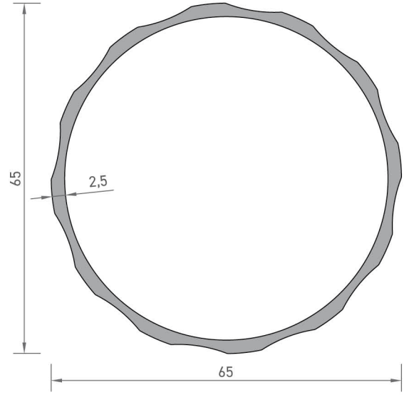
3048 BORU PROFİLİ 1,100 kg/mt
