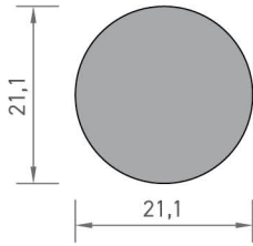
6236 DOLU BORU PROFİLİ 1,916 kg/mt
