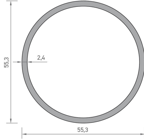
3021 BORU PROFİLİ 1,090 kg/mt
