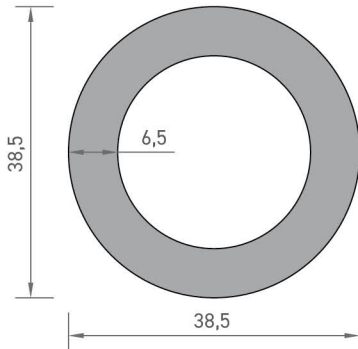
8830 BORU PROFİLİ 1,771 kg/mt
