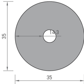
3016 BORU PROFİLİ 2,520 kg/mt
