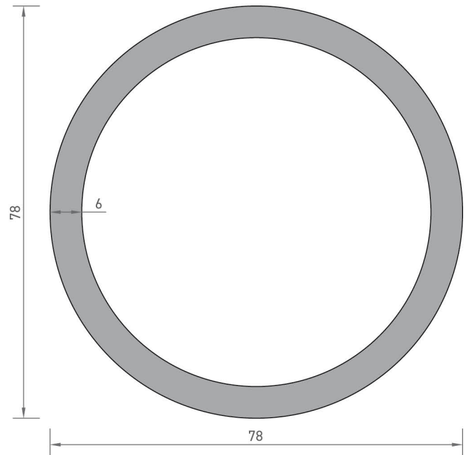
6883 BORU PROFİLİ 3,680 kg/mt
