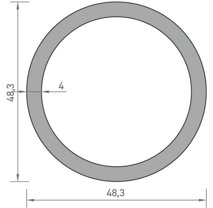
3752 BORU PROFİLİ 1,510 kg/mt
