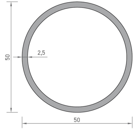
3753 BORU PROFİLİ 1,011 kg/mt
