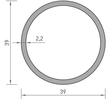
2981 BORU PROFİLİ 0,690 kg/mt
