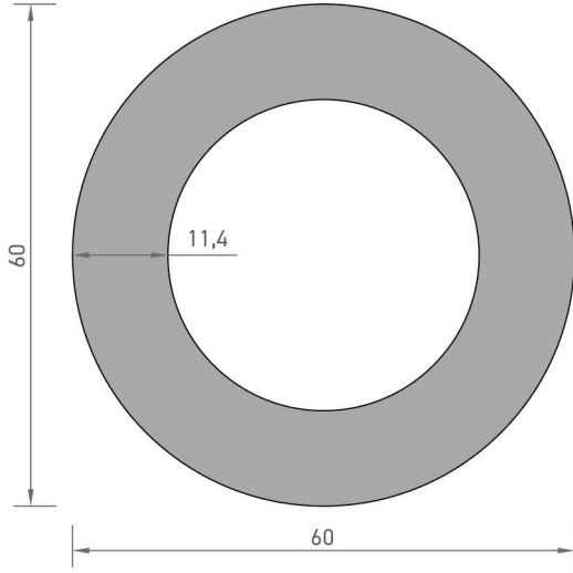
8091 BORU PROFİLİ 4,720 kg/mt
