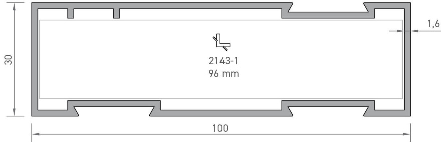
2147 GENİŞ KASA PROFİLİ 1,215 kg/mt
