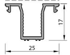
8 MM CAM ÇITA PROFİL V.ES.115 0.178 kg/mt
